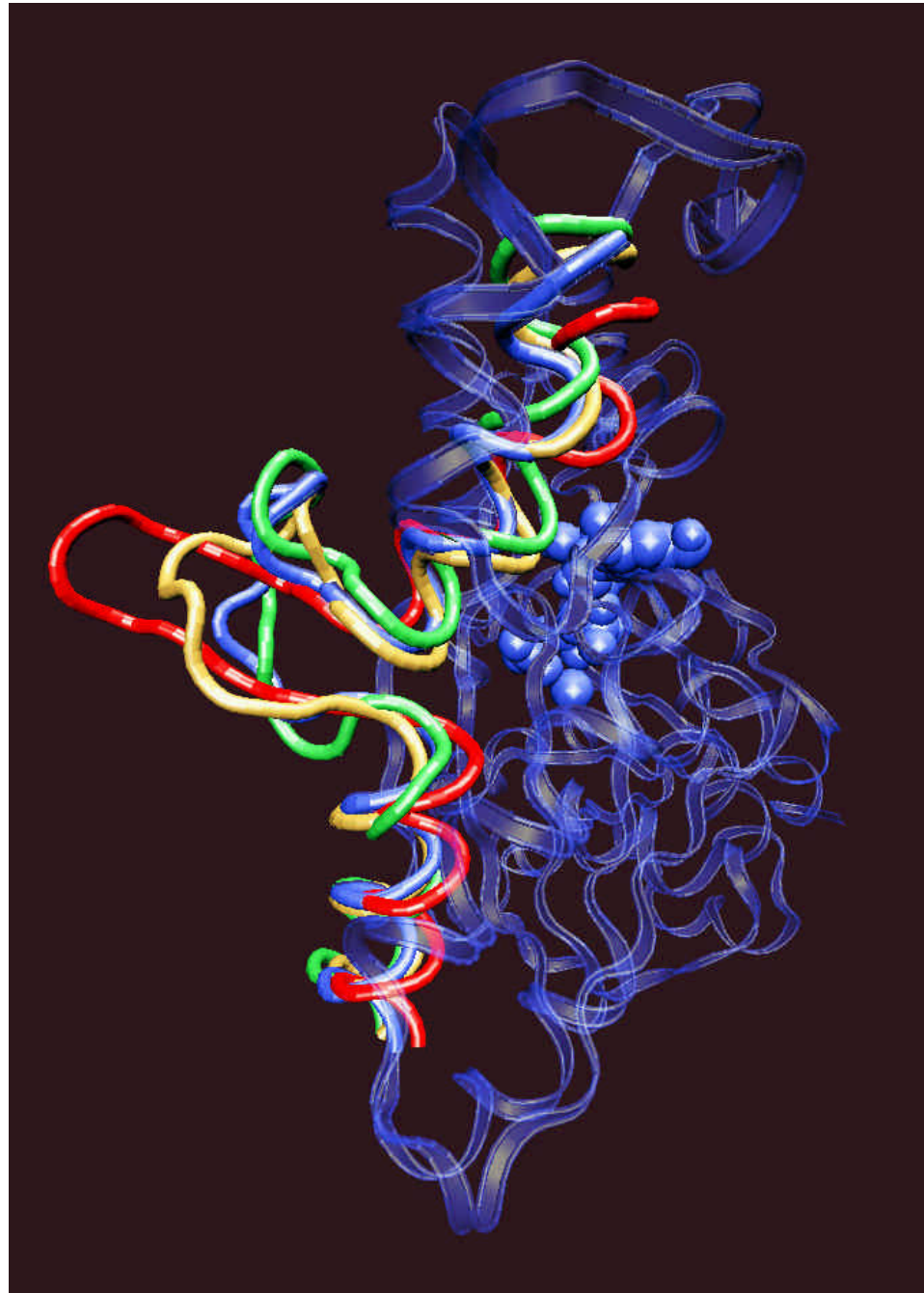
FIGURE 10 Conformation of the "hydrophobic plug" loop 264–273 in four structures aligned with the Kabach crystal structure (KAT), visualized by VMD (Humphrey et al., 1996). The backbone of residues 253–285 is shown as a colored tube in each case. Green , final structure of CDC; blue , KAT; red , LOR; brown , final structure of CTM. The protein backbone is shown in transparent ribbon representation; ATP and divalent cations are represented by van der Waals spheres.
