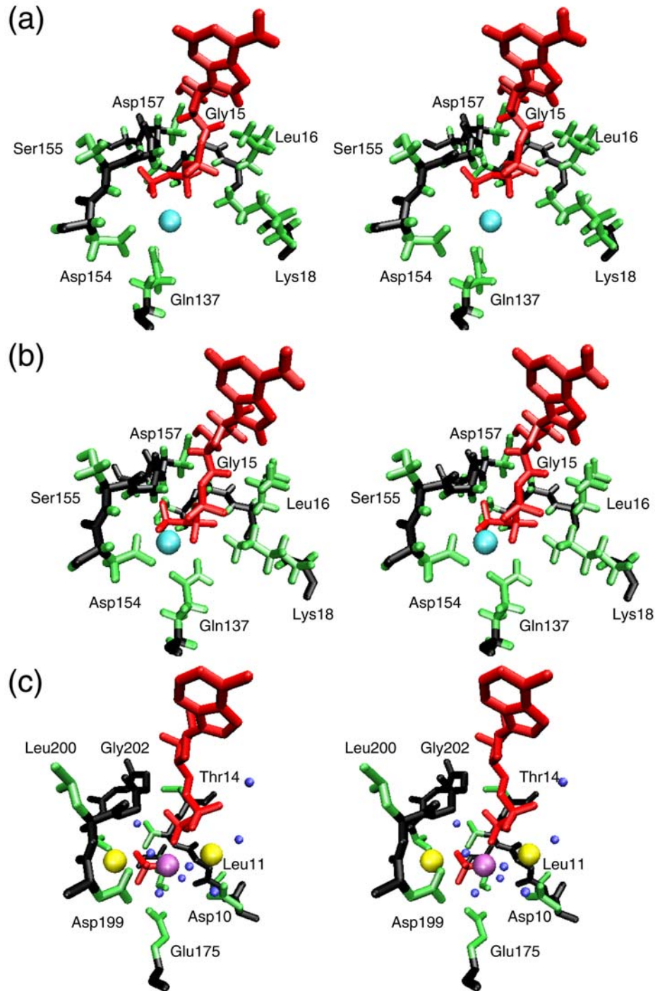
FIGURE 4 Comparison of nucleotide binding sites, visualized by VMD (Humphrey et al., 1996). The nucleotides are shown in red. Ions are represented as spheres: \text{Ca}^{2+} in cyan, \text{Mg}^{2+} in purple, and \text{K}^{+} in yellow. Water oxygens are shown as small blue spheres. The protein backbone is presented in black, and side chains are green. (a) ATP binding site of the Kabsch crystal structure (Kabsch et al., 1990). (b) ATP binding site of the final structures of CTC. (c) ADP- \text{P}_i binding site of the chaperone Hsc70 (Wilbanks and McKay, 1995).
